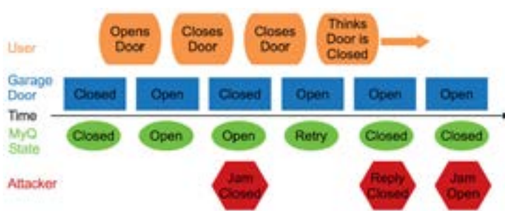
Figure 1: Attack timeline
